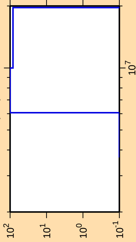
\Delta\sigma/\sigma vs. E for ^{73}\text{Se}(n,d)
