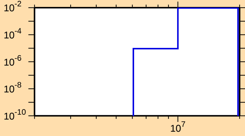
\sigma vs. E for ^{73}\text{Se}(n,d)
