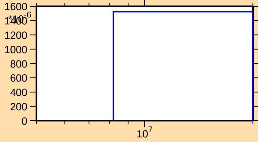
\sigma vs. E for ^{78}\text{Se}(n,np)
