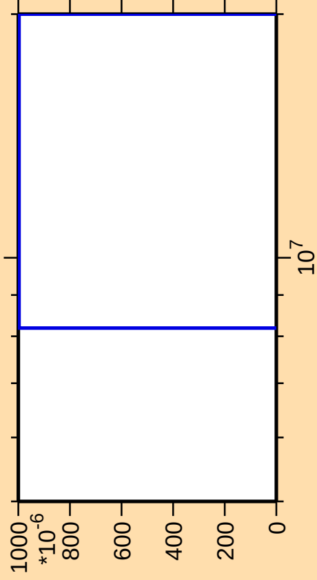
\Delta\sigma/\sigma vs. E for ^{78}\text{Se}(n,\text{pd})
