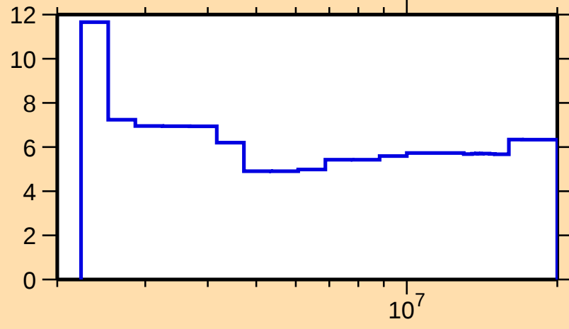
\Delta\sigma/\sigma vs. E for ^{81}\text{Se}(n,n\text{nonel.})
