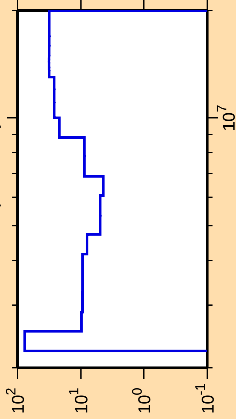
\Delta\sigma/\sigma vs. E for ^{81}\text{Se}(n,\text{ncont.})
