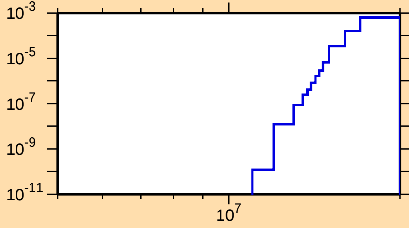
\sigma vs. E for ^{81}\text{Se}(n,n\alpha)
