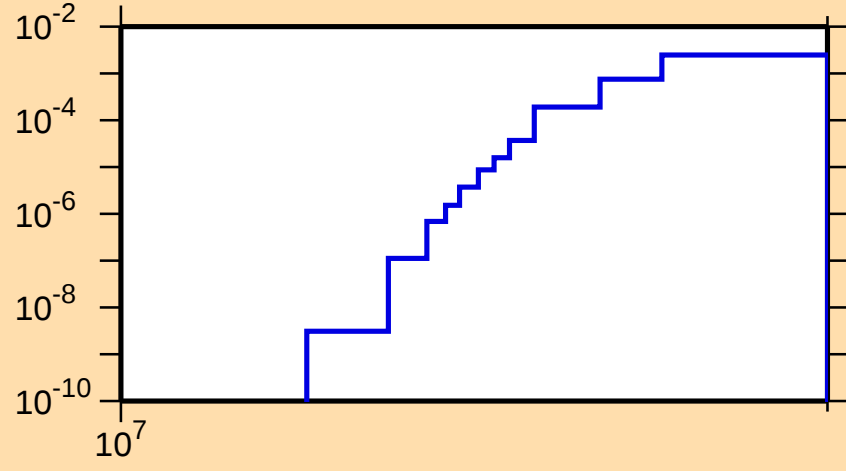
\sigma vs. E for ^{81}\text{Se}(n,np)
