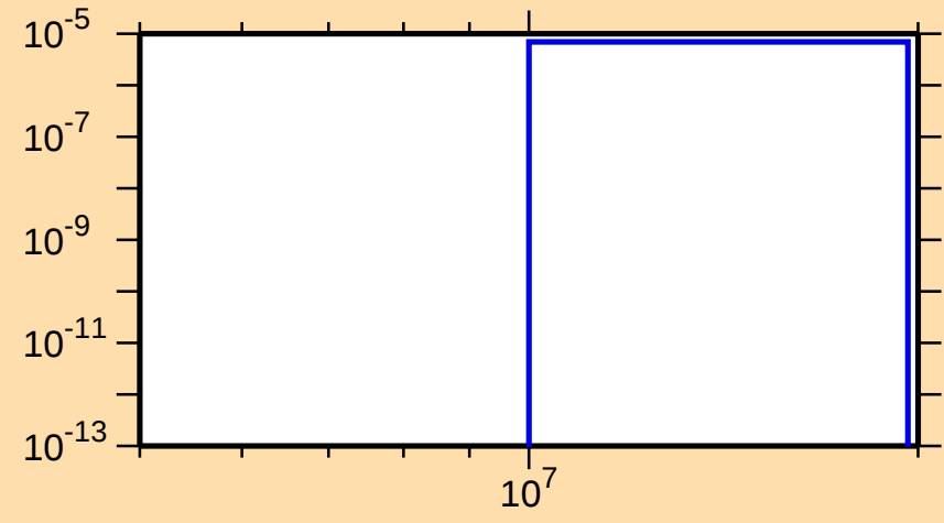
\sigma vs. E for ^{83}\text{Se}(n,t)
