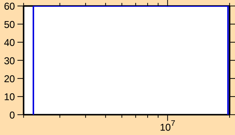
\Delta\sigma/\sigma vs. E for ^{83}\text{Se}(n,\gamma)
