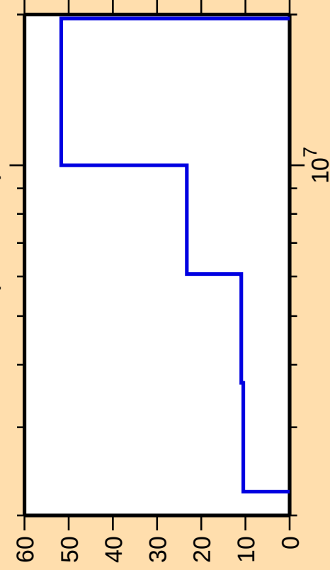
\Delta\sigma/\sigma vs. E for ^{83}\text{Se}(n,\text{ncont.})
