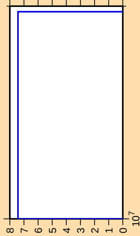
\Delta\sigma/\sigma vs. E for ^{83}\text{Se}(n,2np)
