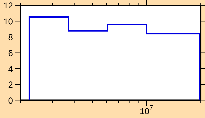
\Delta\sigma/\sigma vs. E for ^{83}\text{Se}(n,n\text{oncl.})
