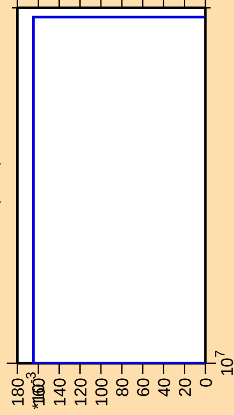
\Delta\sigma/\sigma vs. E for ^{83}\text{Se}(n,\text{nt})
