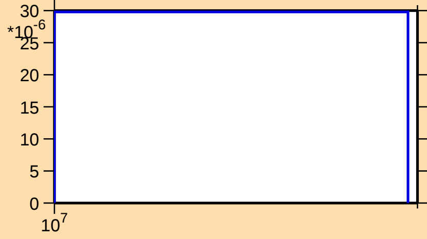
\sigma vs. E for ^{83}\text{Se}(n,d)
