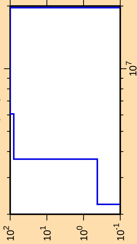
\Delta\sigma/\sigma vs. E for ^{83}\text{Se}(n,\alpha)
