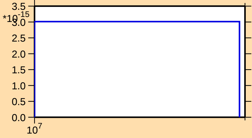
\sigma vs. E for ^{83}\text{Se}(n,\text{nt})
