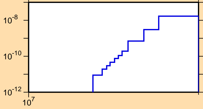
\sigma vs. E for ^{265}\text{He3} )
