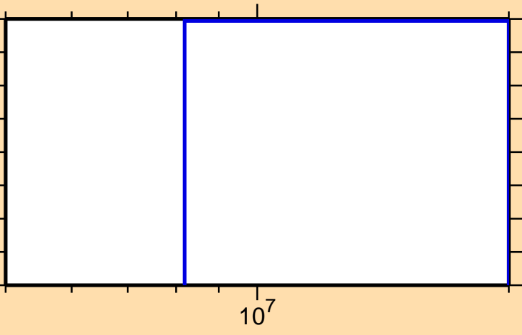
\sigma vs. E for ^{265}
