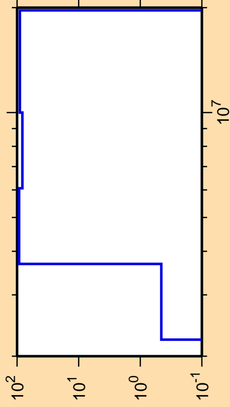
\Delta\sigma/\sigma vs. E for ^{268}_{1}
