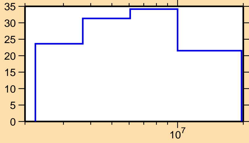
\Delta\sigma/\sigma vs. E for ^{269}\text{Pu}
