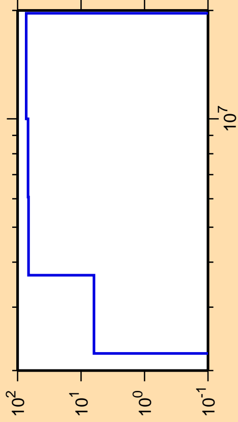
\Delta\sigma/\sigma vs. E for ^{269}\text{Pu}
