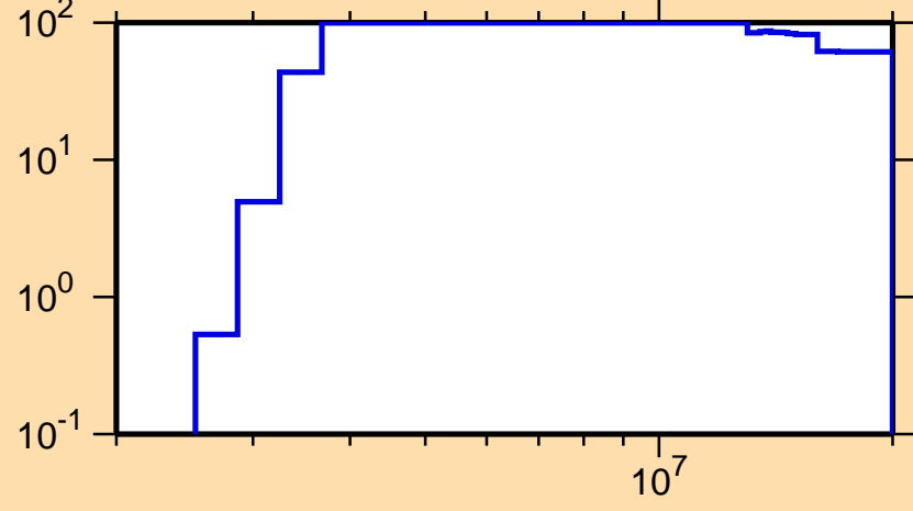
\Delta\sigma/\sigma vs. E for ^{271}
