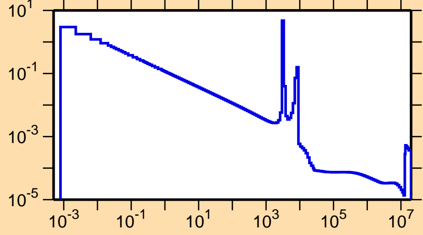
\sigma vs. E for ^{26}\text{Si}(n,\gamma)
