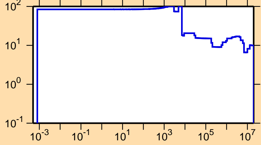
\Delta\sigma/\sigma vs. E for ^{26}\text{Si}(n,\text{el.})
