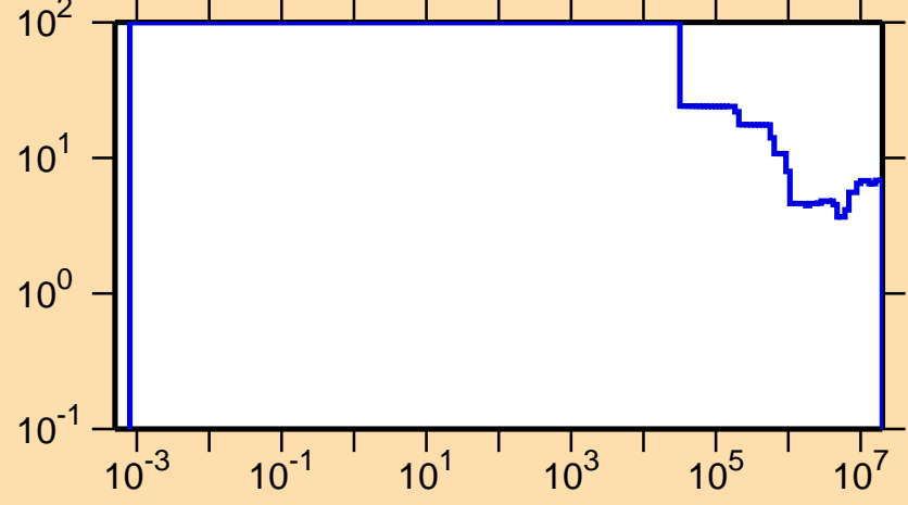
\Delta\sigma/\sigma vs. E for ^{26}\text{Si}(n,\text{nonel.})
