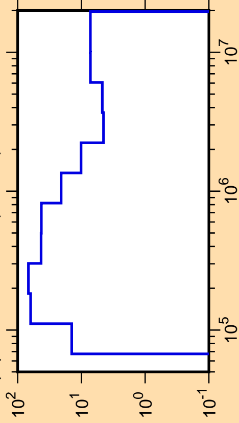
\Delta\mu/\mu vs. E for ^{26}\text{Si}(\text{mt251})
