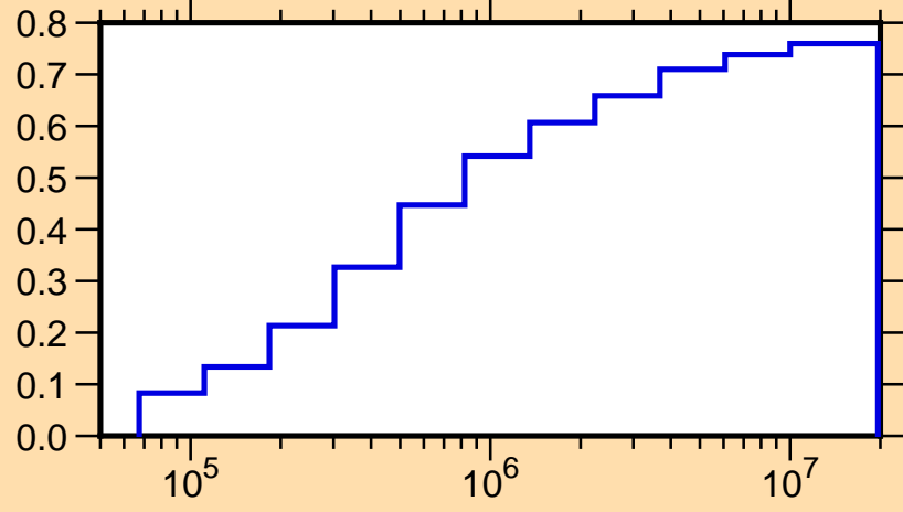
\mu vs. E for ^{26}\text{Si}(\text{mt251})
