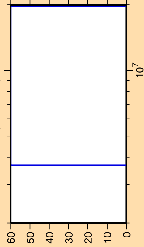
\Delta\sigma/\sigma vs. E for ^{26}\text{Si}(n,\text{ncont.})
