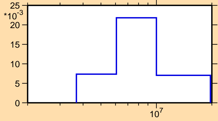
\sigma vs. E for ^{26}\text{Si}(n,n\text{cont.})
