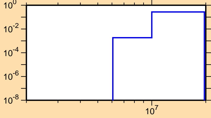
\sigma vs. E for ^{26}\text{Si}(n,p\alpha)
