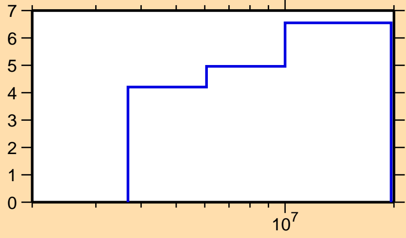
\Delta\sigma/\sigma vs. E for ^{26}\text{Si}(n,n\text{nonel.})
