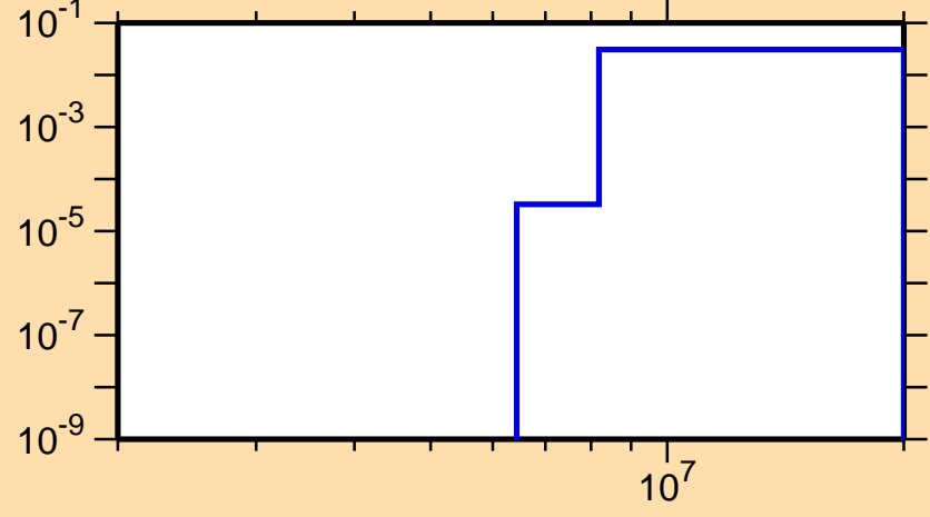
\sigma vs. E for ^{26}\text{Si}(n,pd)
