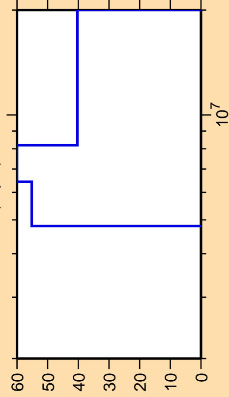
\Delta\sigma/\sigma vs. E for ^{26}\text{Si}(n,pd)
