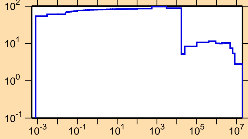
\Delta\sigma/\sigma vs. E for ^{26}\text{Si}(n,\text{tot.})
