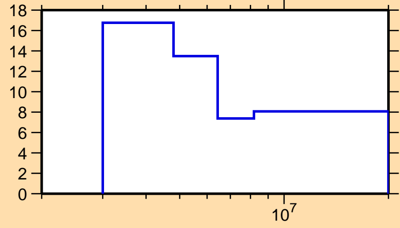
\Delta\sigma/\sigma vs. E for ^{26}\text{Si}(n,el.)
