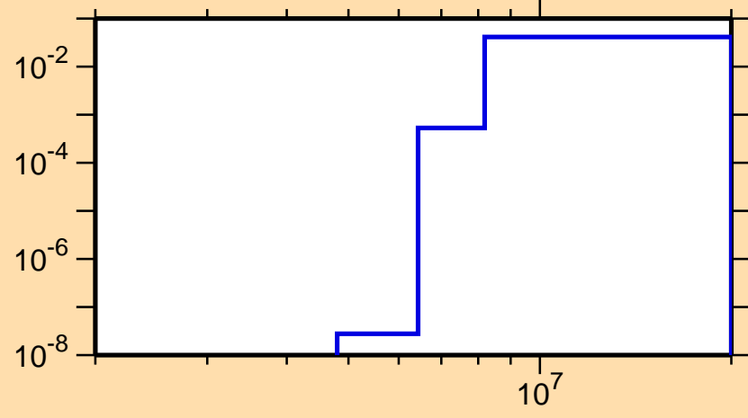
\sigma vs. E for ^{26}\text{Si}(n,np)
