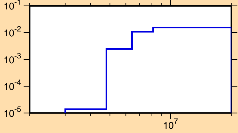
\sigma vs. E for ^{26}\text{Si}(n,d)
