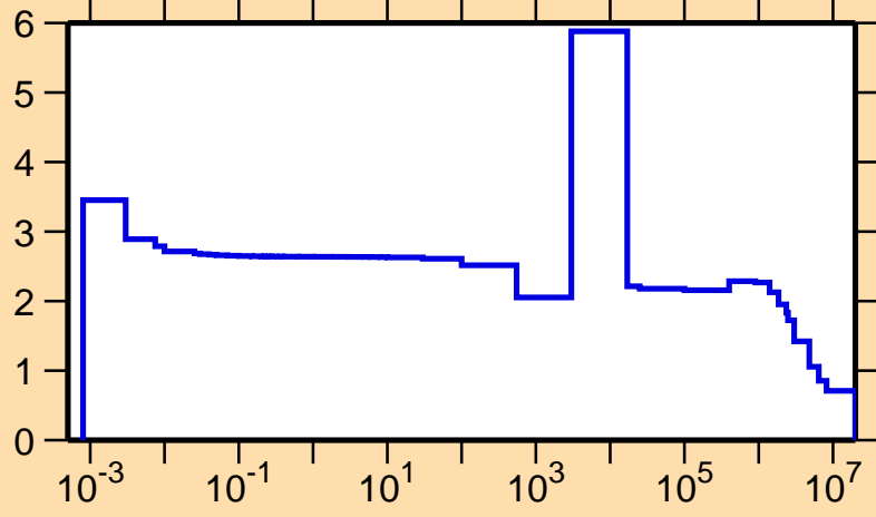
\sigma vs. E for ^{26}\text{Si}(n,\text{el.})
