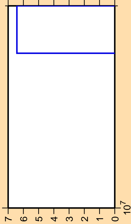
\Delta\sigma/\sigma vs. E for ^{27}\text{Si}(\text{mt } 45)
