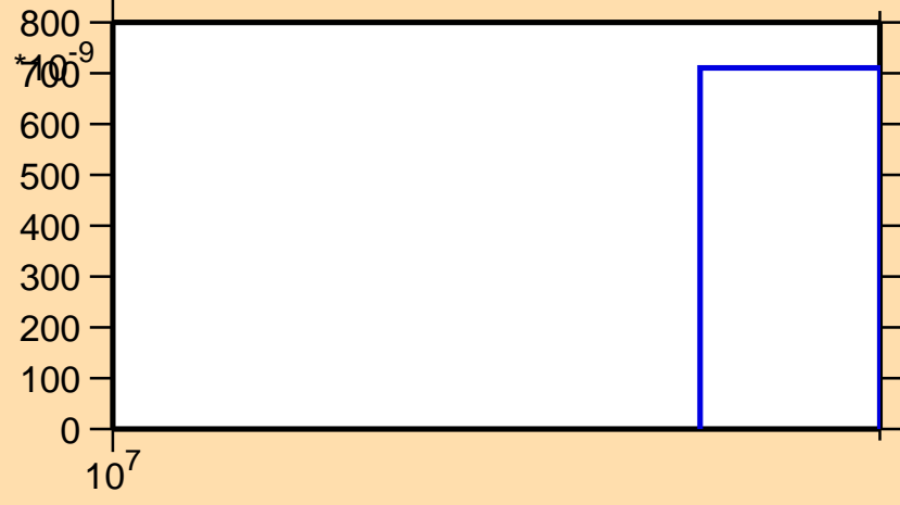
\sigma vs. E for ^{27}\text{Si}(n,\text{nd})
