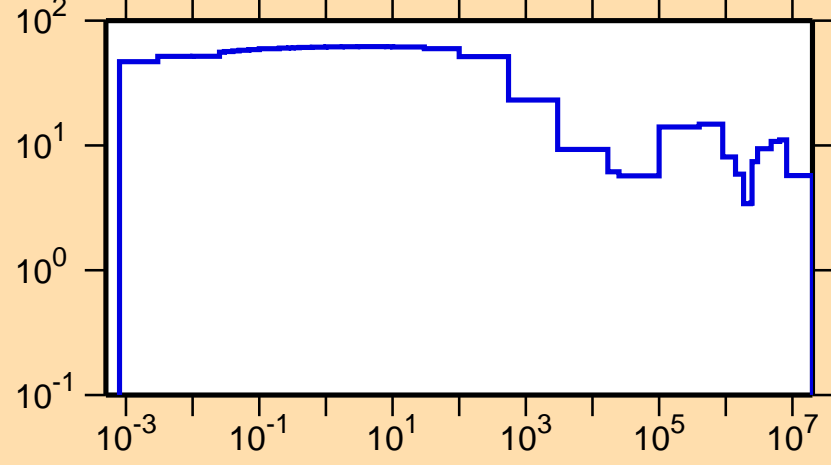
\Delta\sigma/\sigma vs. E for ^{27}\text{Si}(n,\text{tot.})
