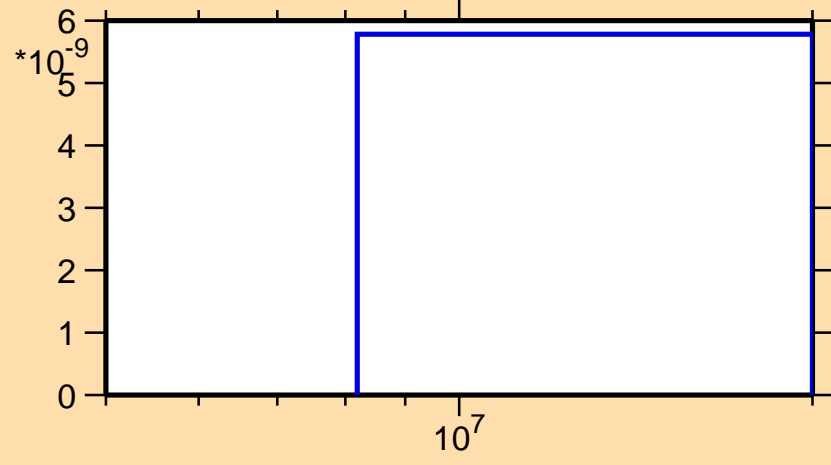
\sigma vs. E for ^{27}\text{Si}(n,\text{nd})
