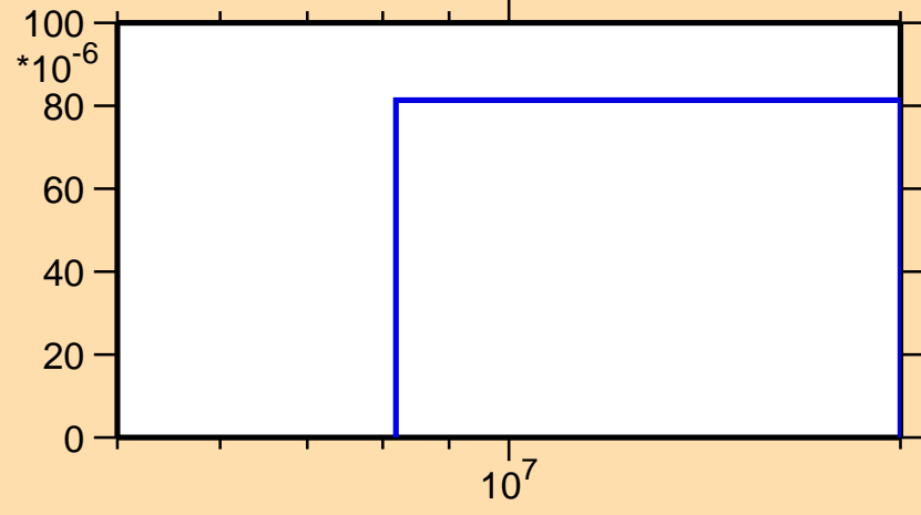
\sigma vs. E for ^{27}\text{Si}(n,t)
