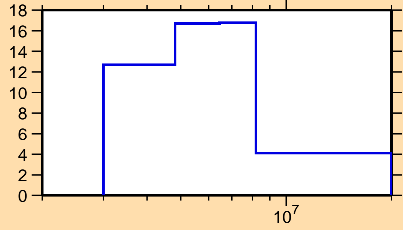
\Delta\sigma/\sigma vs. E for ^{27}\text{Si}(n,el.)
