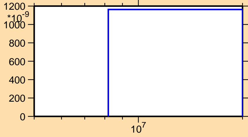
\sigma vs. E for ^{27}\text{Si}(\text{mt } 34)
