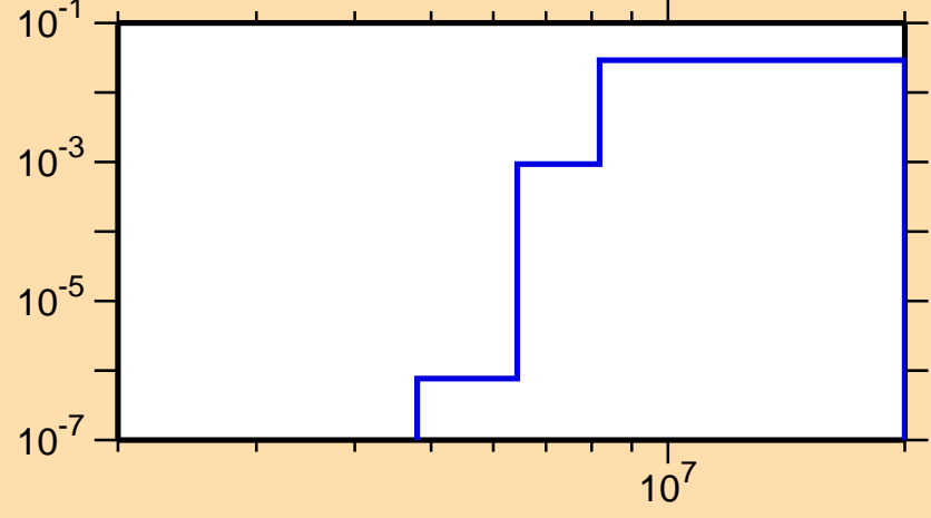
\sigma vs. E for ^{27}\text{Si}(n,d)
