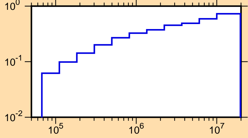
\mu vs. E for ^{28}\text{Si}(\text{mt251})
