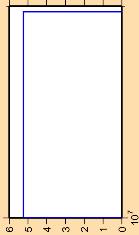
\Delta\sigma/\sigma vs. E for ^{28}\text{Si}(n,\text{pd})
