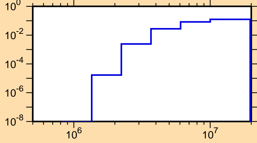
\sigma vs. E for ^{29}\text{Si}(n,\alpha)
