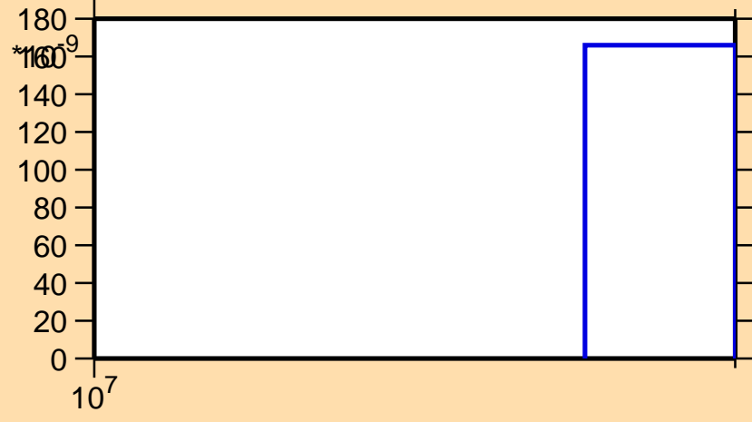
\sigma vs. E for ^{31}\text{Si}(n,\text{nd})
