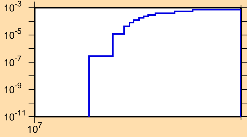
\sigma vs. E for ^{31}\text{Si}(n,t)
