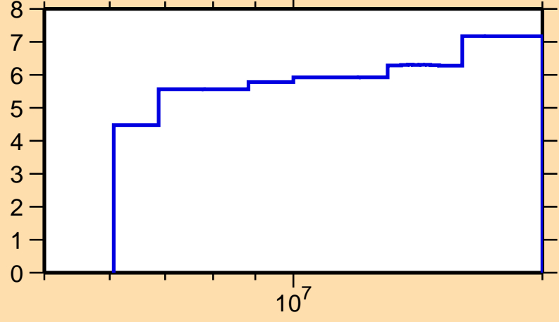
\Delta\sigma/\sigma vs. E for ^{31}\text{Si}(n,\text{nonel.})
