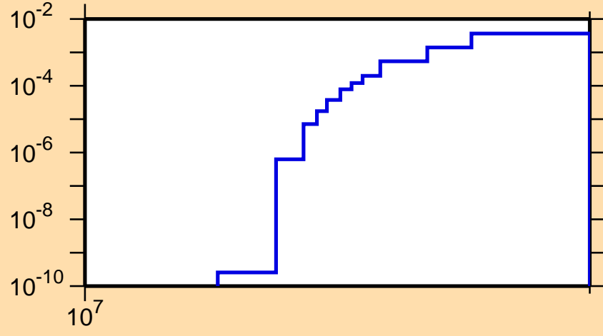
\sigma vs. E for ^{31}\text{Si}(n,d)
