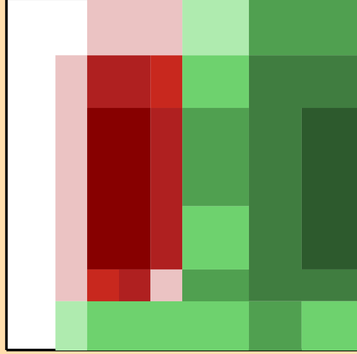
\Delta\sigma/\sigma vs. E for ^{31}\text{Si}(n,2n)
