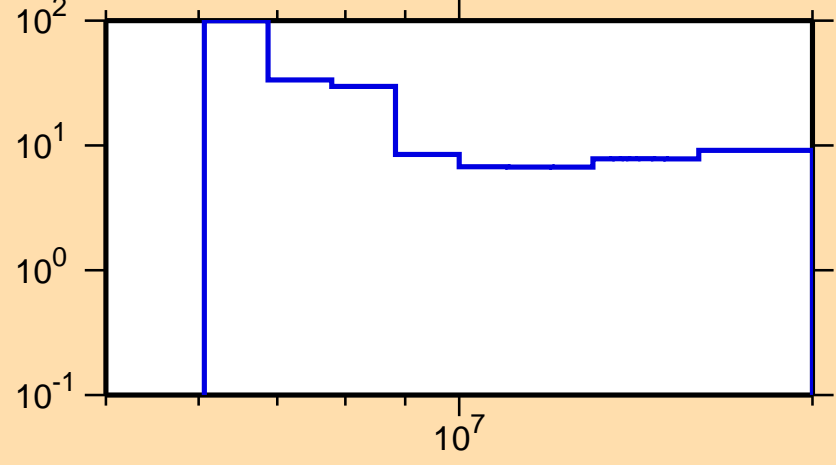
\Delta\sigma/\sigma vs. E for ^{31}\text{Si}(n,2n)
