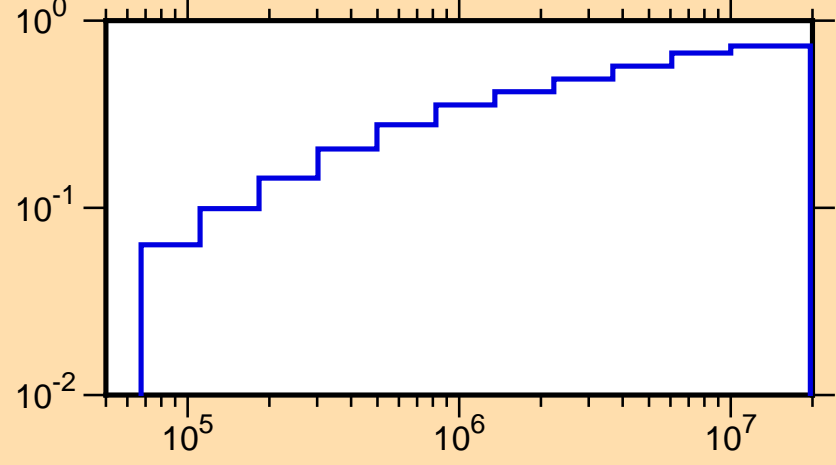
\mu vs. E for ^{31}\text{Si}(\text{mt251})
