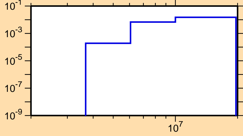
\sigma vs. E for ^{31}\text{Si}(n,\alpha)
