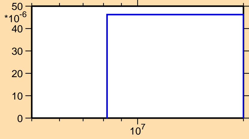
\sigma vs. E for ^{31}\text{Si}(n,np)
