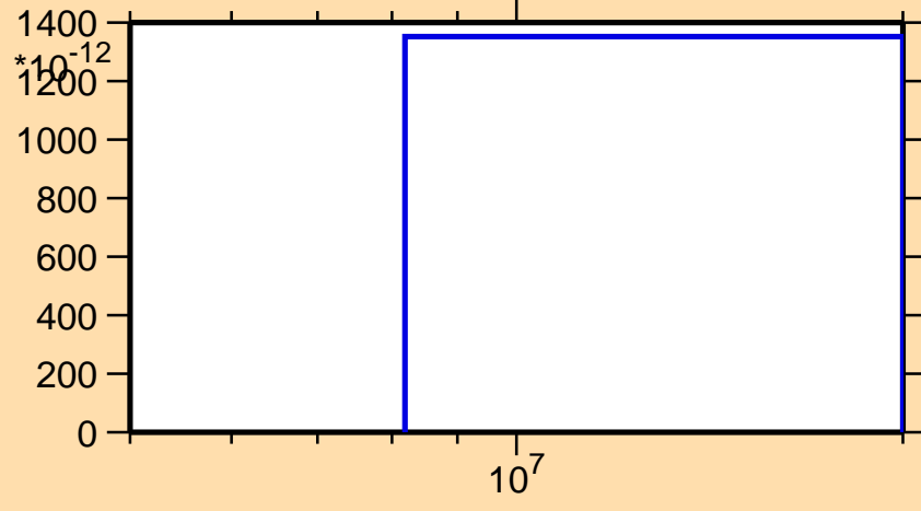
\sigma vs. E for ^{31}\text{Si}(n,\text{nd})
