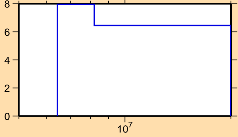
\Delta\sigma/\sigma vs. E for ^{31}\text{Si}(n,\text{el.})
