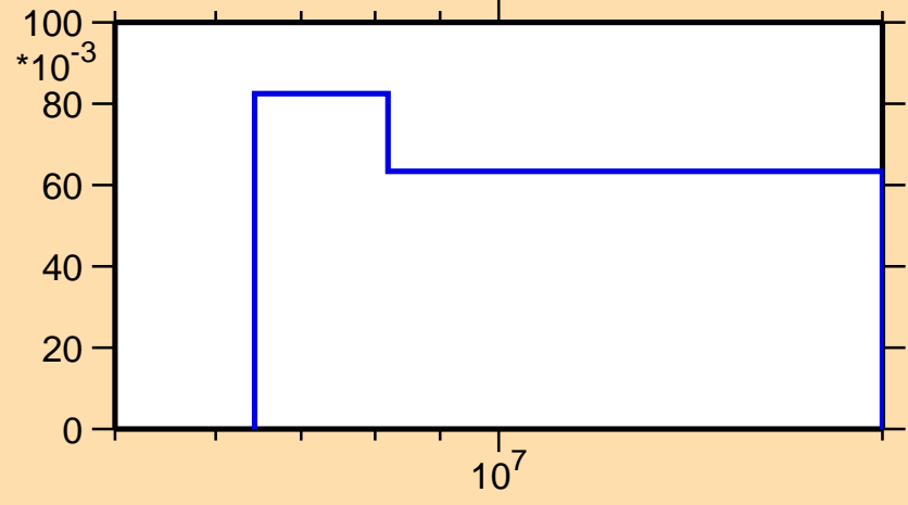
\sigma vs. E for ^{31}\text{Si}(n,n\text{cont.})
