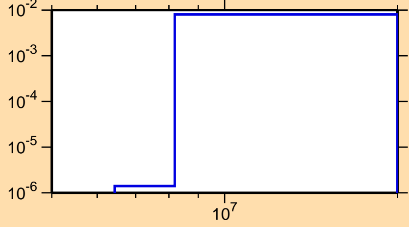
\sigma vs. E for ^{31}\text{Si}(n,p)
