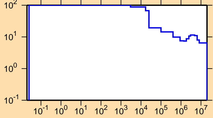
\Delta\sigma/\sigma vs. E for ^{31}\text{Si}(n,\text{el.})
