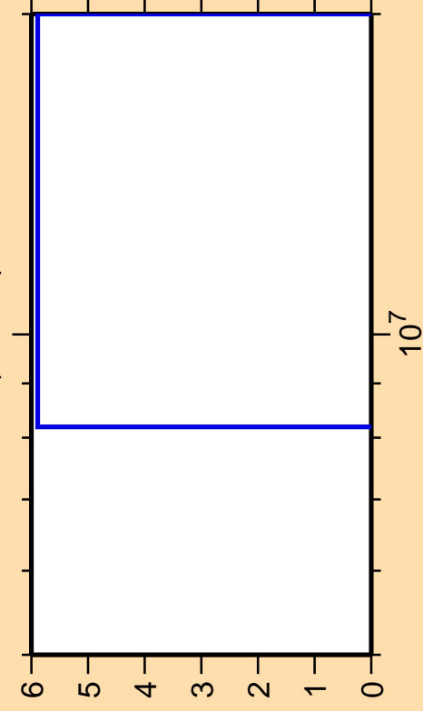
\Delta\sigma/\sigma vs. E for ^{31}\text{Si}(n,2n\alpha)
