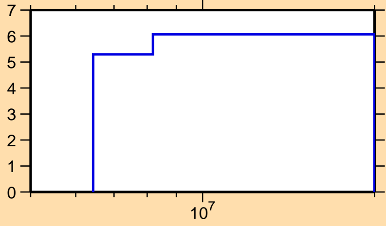
\Delta\sigma/\sigma vs. E for ^{31}\text{Si}(n,n\text{nonel.})
