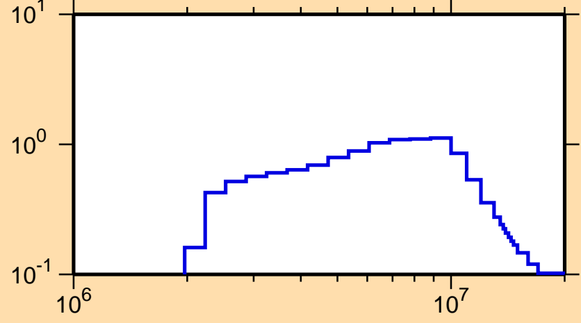
\sigma vs. E for ^{32}\text{Si}(n,\text{inel.})
