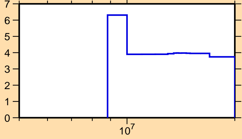
\Delta\sigma/\sigma vs. E for ^{32}\text{Si}(n,\text{tot.})
