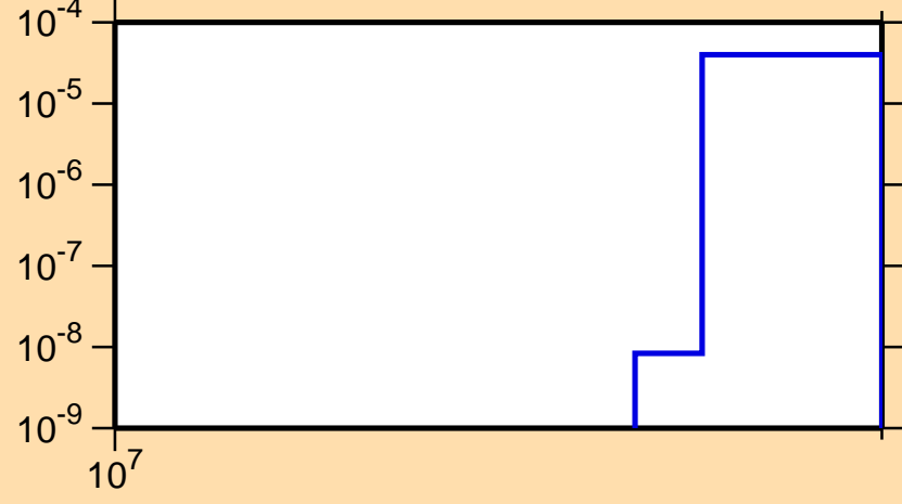
\sigma vs. E for ^{32}\text{Si}(n,np)
