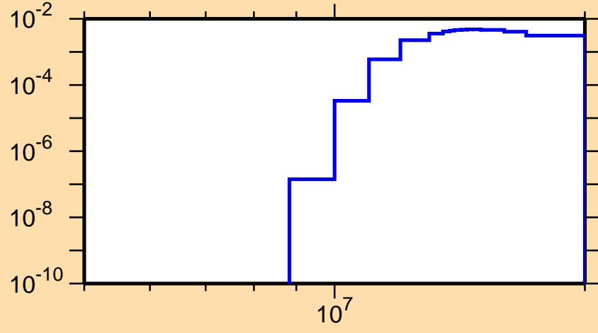
\sigma vs. E for ^{32}\text{Si}(n,\alpha)
