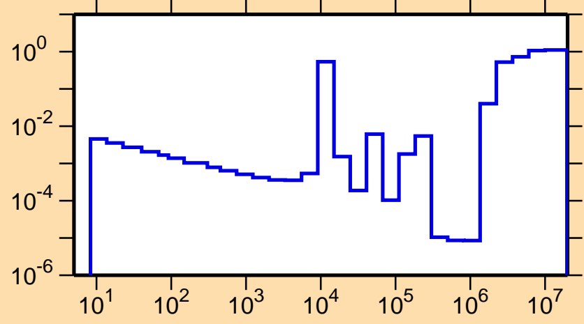
\sigma vs. E for ^{32}\text{Si}(n,\text{nonel.})
