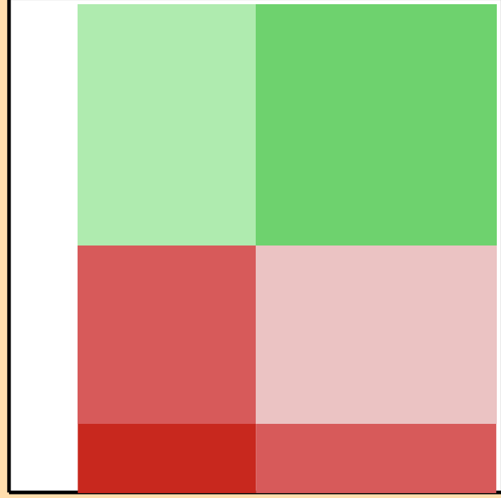
\Delta\sigma/\sigma vs. E for ^{32}\text{Si}(n,n\text{cont.})
