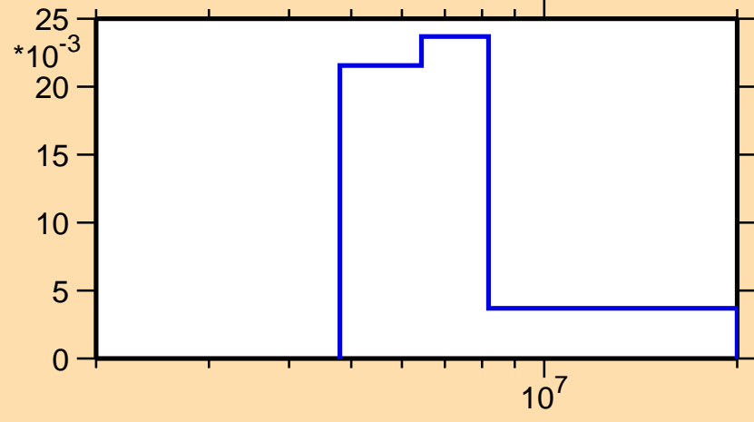
\sigma vs. E for ^{32}\text{Si}(n,n_3)
