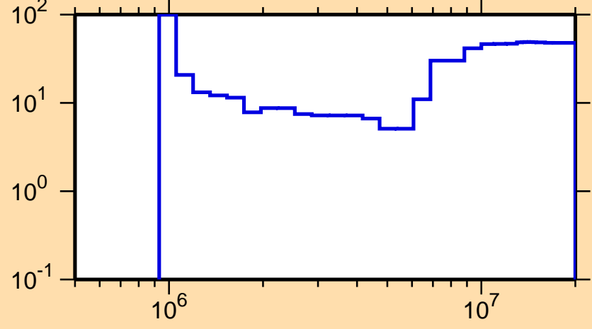
\Delta\sigma/\sigma vs. E for ^{33}\text{Si}(n,\text{inel.})
