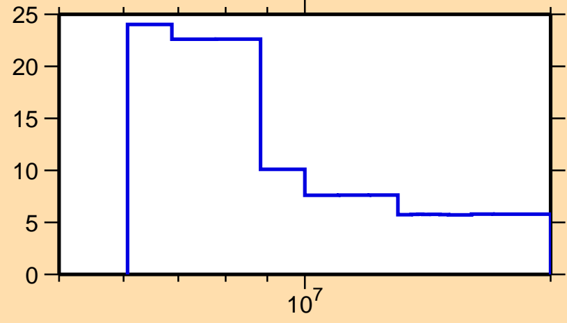
\Delta\sigma/\sigma vs. E for ^{33}\text{Si}(n,el.)
