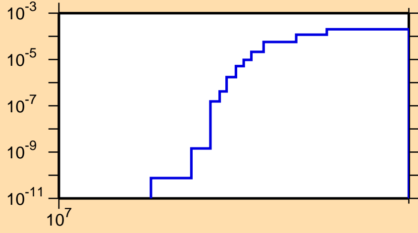
\sigma vs. E for ^{33}\text{Si}(n,t)
