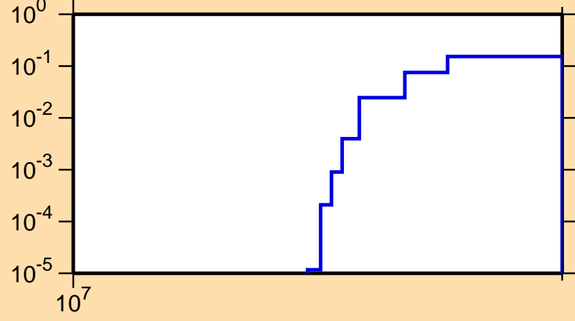
\sigma vs. E for ^{33}\text{Si}(n,3n)
