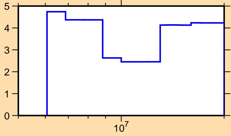
\Delta\sigma/\sigma vs. E for ^{33}\text{Si}(n,n\text{nonel.})
