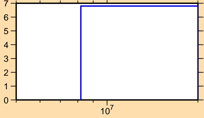
\Delta\sigma/\sigma vs. E for ^{33}\text{Si}(n,2n)
