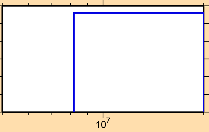
\sigma vs. E for ^{33}\text{Si}(n,\text{nd})
