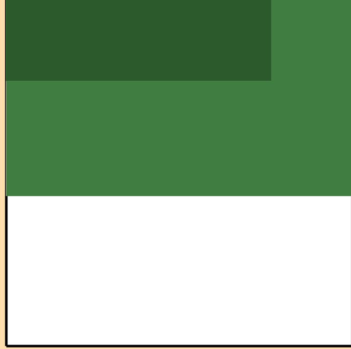
\Delta\sigma/\sigma vs. E for ^{34}\text{Si}(n,\text{el.})
