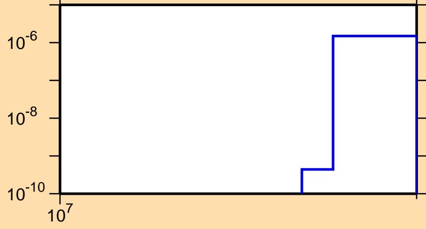
\sigma vs. E for ^{34}\text{Si}(n,t)
