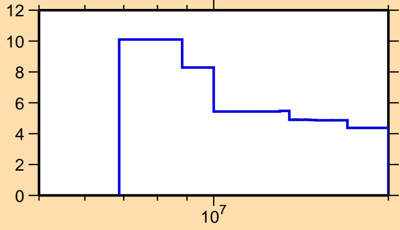
\Delta\sigma/\sigma vs. E for ^{34}\text{Si}(n,tot.)
