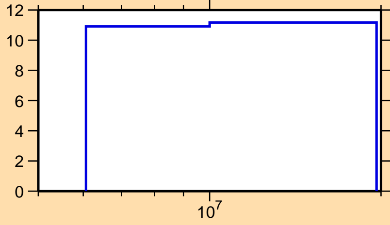
\Delta\sigma/\sigma vs. E for ^{34}\text{Si}(n,n\text{onel.})
