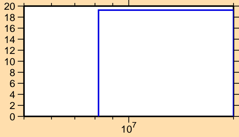
\Delta\sigma/\sigma vs. E for ^{34}\text{Si}(n,ncont.)
