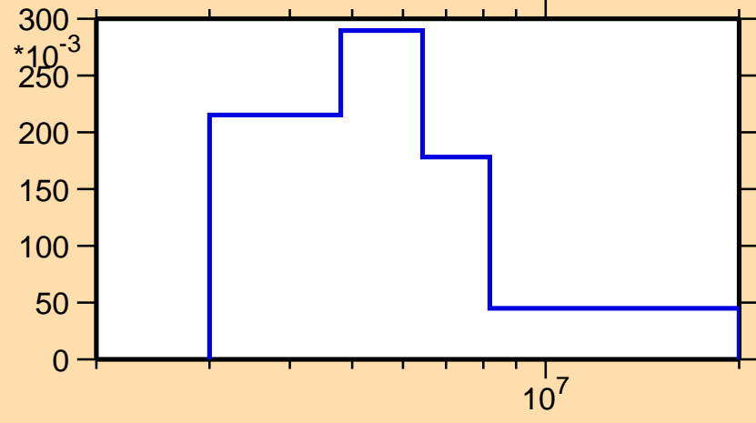
\sigma vs. E for ^{34}\text{Si}(n,n_1)
