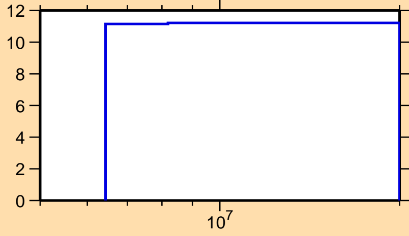
\Delta\sigma/\sigma vs. E for ^{34}\text{Si}(n,n\text{nonel.})
