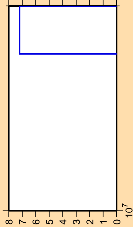
\Delta\sigma/\sigma vs. E for ^{100}\text{Sn}(n,n_1)
