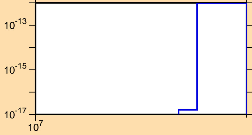
\sigma vs. E for ^{100}\text{Sn}(n,\text{nd})
