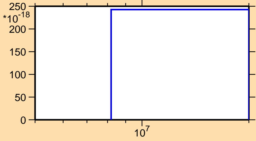
\sigma vs. E for ^{100}\text{Sn}(n,2np)
