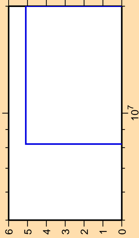
\Delta\sigma/\sigma vs. E for ^{100}\text{Sn}(\text{mt } 34)
