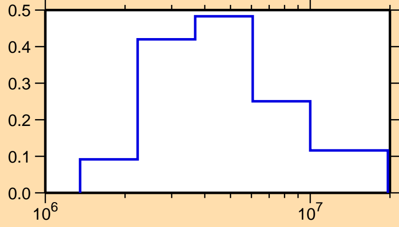
\sigma vs. E for ^{102}\text{Sn}(n,\text{inel.})
