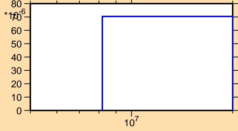
\sigma vs. E for ^{102}\text{Sn}(n,t)
