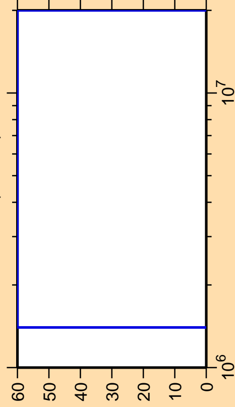
\Delta\sigma/\sigma vs. E for ^{102}\text{Sn}(n,\text{inel.})
