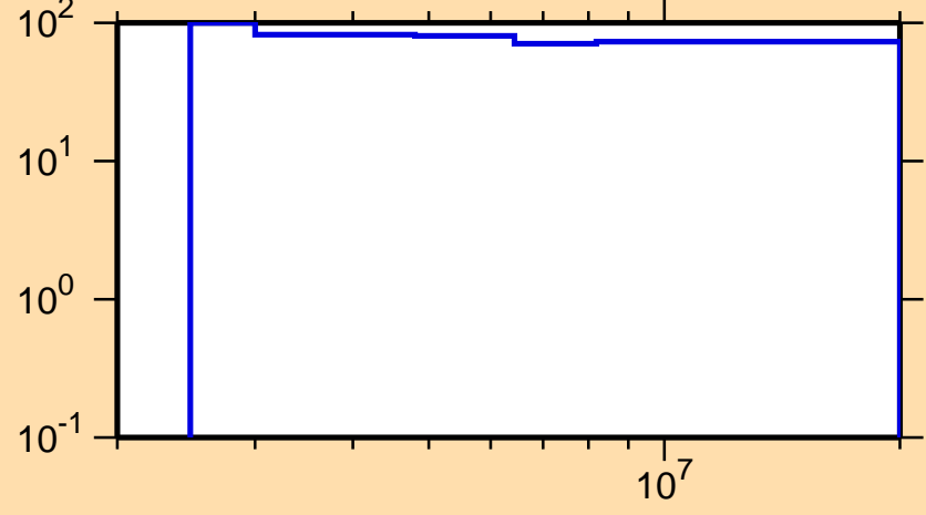
\Delta\sigma/\sigma vs. E for ^{102}\text{Sn}(n,ncont.)
