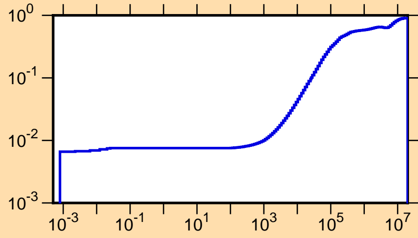
\mu vs. E for ^{103}\text{Sn}(\text{mt251})
