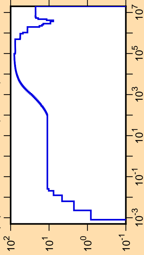
\Delta\mu/\mu vs. E for ^{103}\text{Sn}(\text{mt251})
