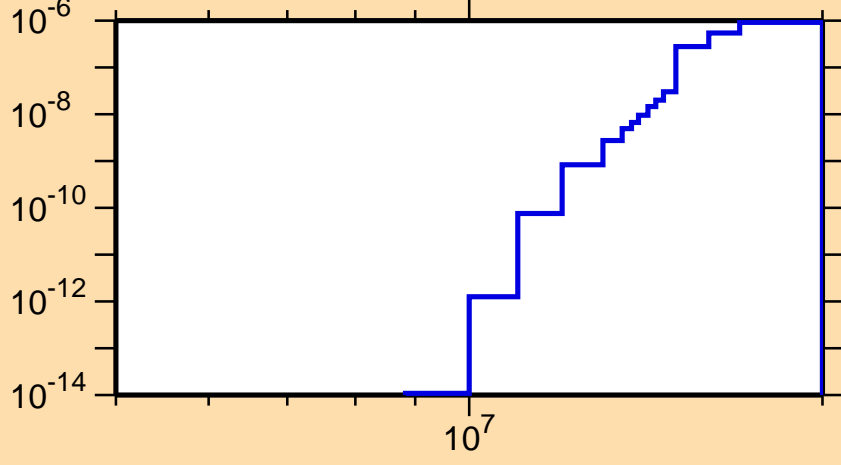
\sigma vs. E for ^{103}\text{Sn}(\text{mt117})
