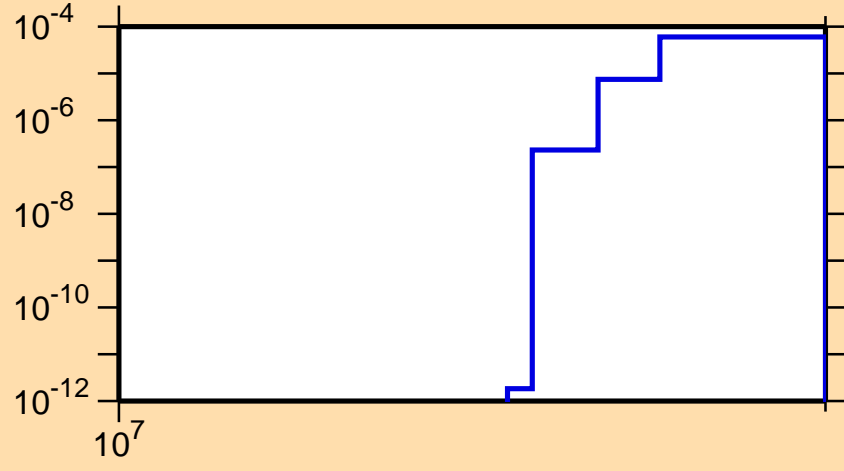
\sigma vs. E for ^{103}\text{Sn}(n,2np)
