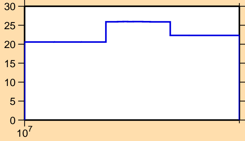
\Delta\sigma/\sigma vs. E for ^{103}\text{Sn}(n,\text{el.})
