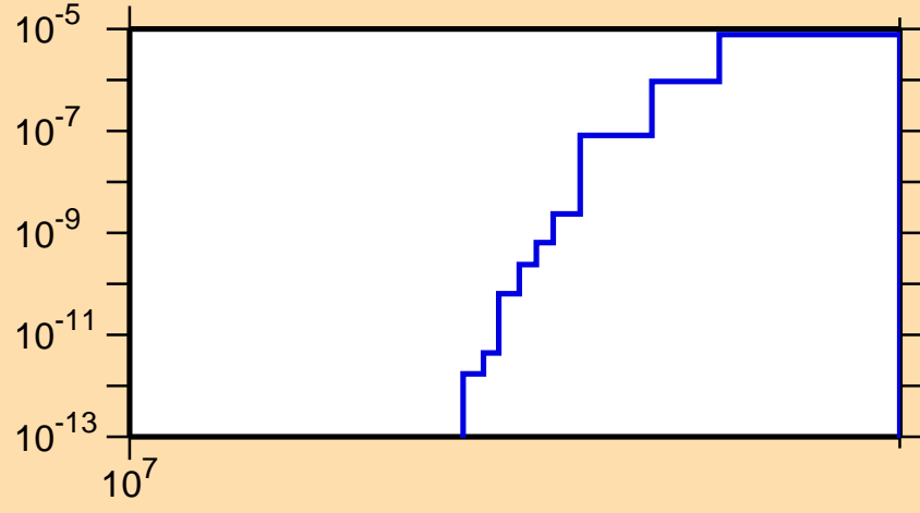
\sigma vs. E for ^{103}\text{Sn}(n,\text{nd})
