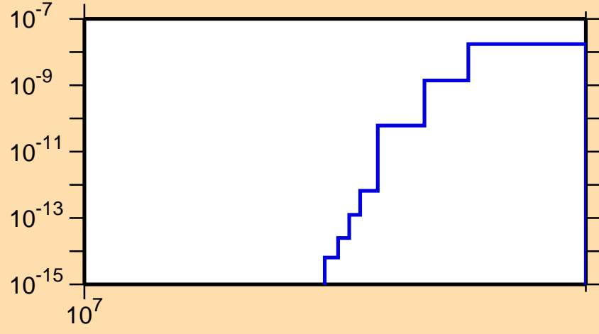
\sigma vs. E for ^{103}\text{Sn}(n,2n\alpha)
