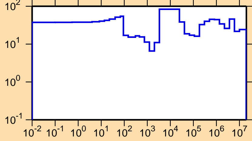
\Delta\sigma/\sigma vs. E for ^{103}\text{Sn}(n,\text{el.})
