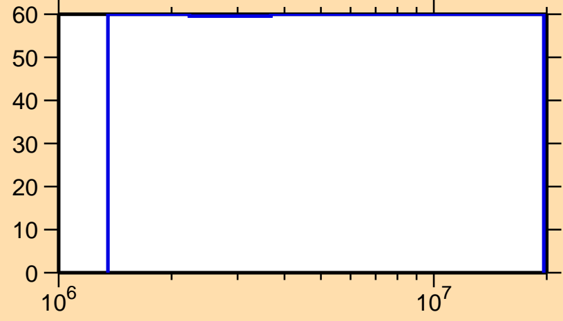
\Delta\sigma/\sigma vs. E for ^{103}\text{Sn}(n,ncont.)
