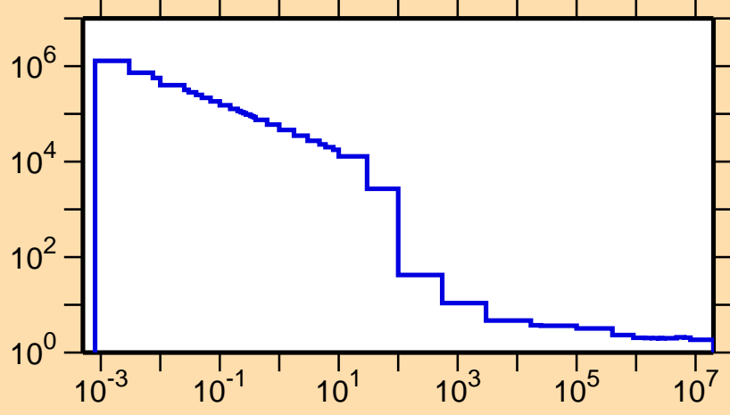
\sigma vs. E for ^{103}\text{Sn}(n,\text{nonel.})
