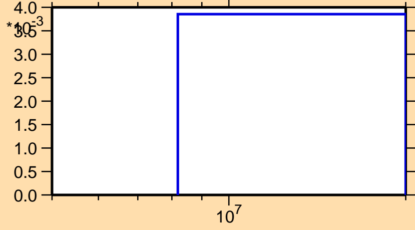
\sigma vs. E for ^{103}\text{Sn}(n,2n)
