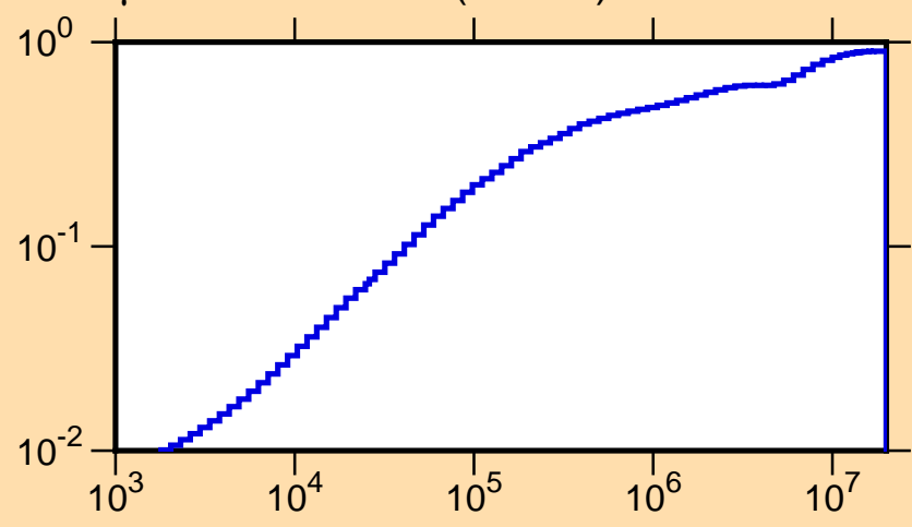
\mu vs. E for ^{104}\text{Sn}(\text{mt251})
