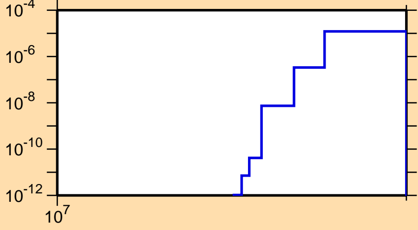
\sigma vs. E for ^{104}\text{Sn}(n,\text{pt})
