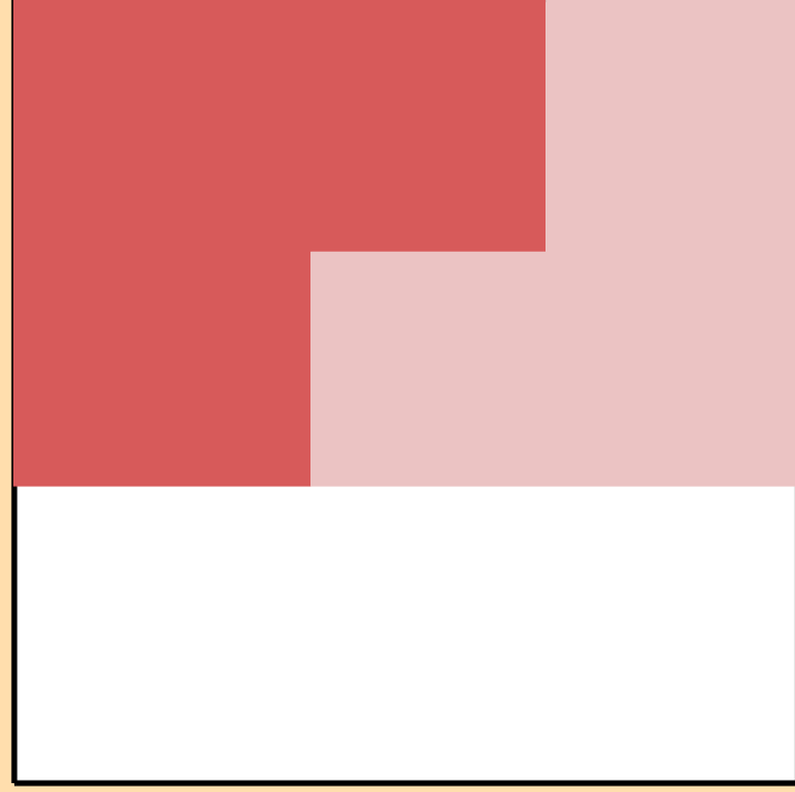
\Delta\sigma/\sigma vs. E for ^{104}\text{Sn}(n,\text{nonel.})
