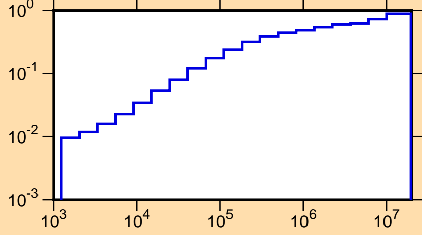
\mu vs. E for ^{104}\text{Sn}(\text{mt251})
