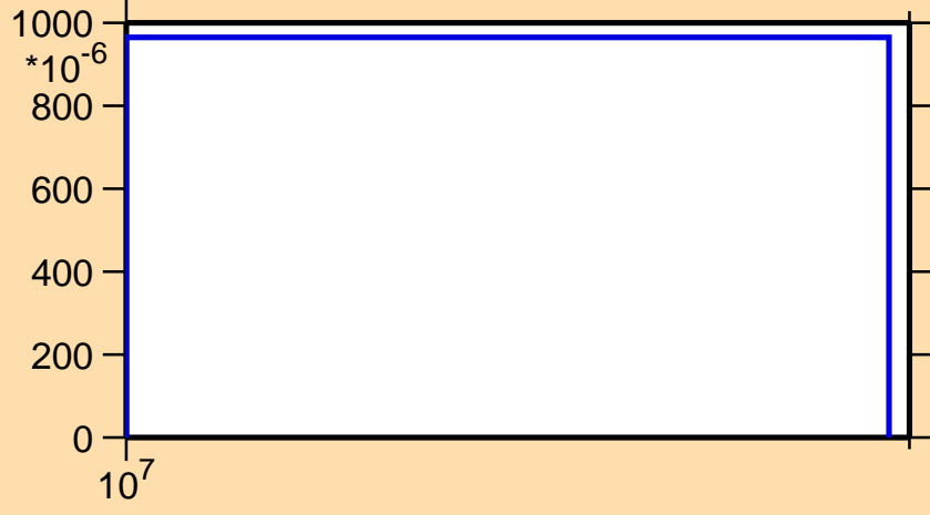
\sigma vs. E for ^{104}\text{Sn}(n,2n)
