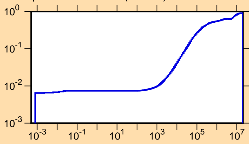
\mu vs. E for ^{105}\text{Sn}(\text{mt251})
