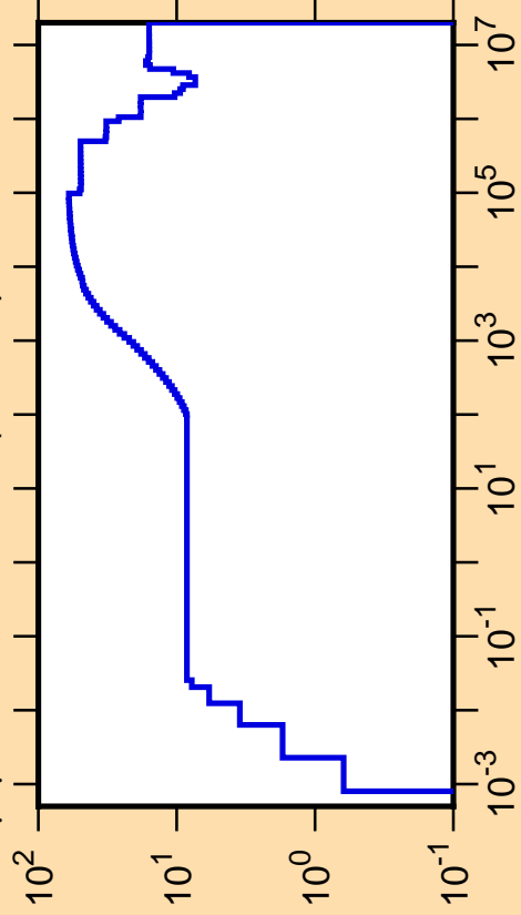
\Delta\mu/\mu vs. E for ^{105}\text{Sn}(\text{mt251})
