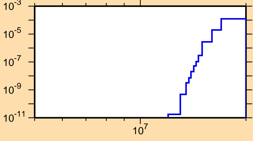
\sigma vs. E for ^{105}\text{Sn}(n,\text{pt})
