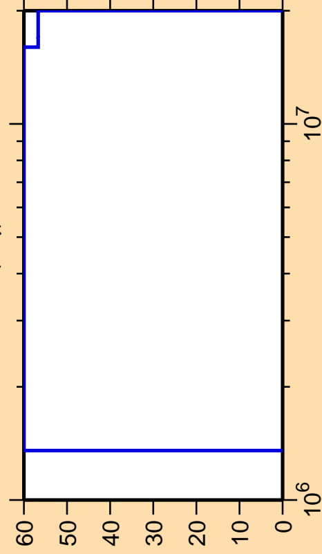
\Delta\sigma/\sigma vs. E for ^{105}\text{Sn}(n,\gamma)
