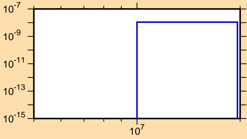
\sigma vs. E for ^{105}\text{Sn}(\text{mt117})
