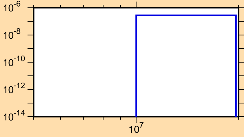
\sigma vs. E for ^{105}\text{Sn}(\text{mt } 45)
