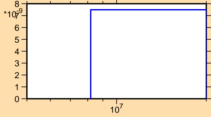
\sigma vs. E for ^{105}\text{Sn}(n,2n\alpha)
