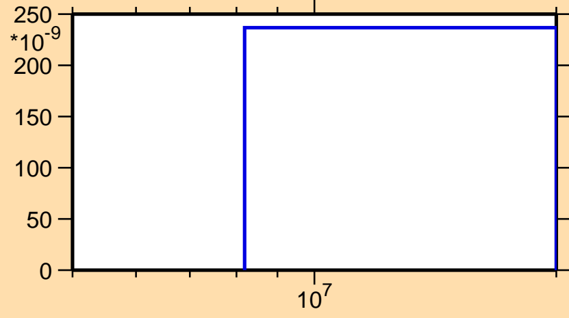
\sigma vs. E for ^{105}\text{Sn}(\text{mt } 45)
