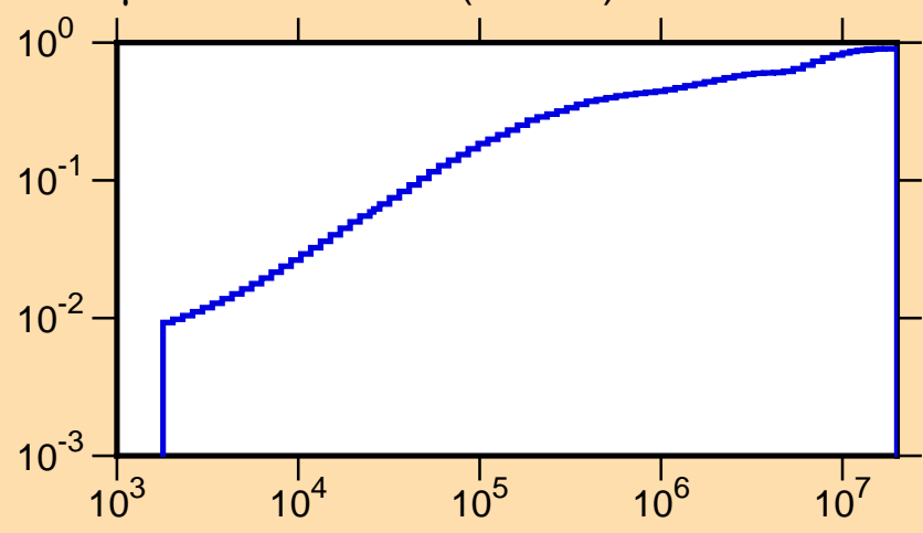
\mu vs. E for ^{106}\text{Sn}(\text{mt251})
