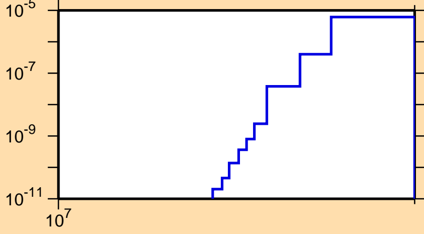
\sigma vs. E for ^{106}\text{Sn} (mt 45)
