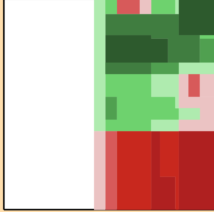
\Delta\sigma/\sigma vs. E for ^{106}\text{Sn}(n,n\text{cont.})
