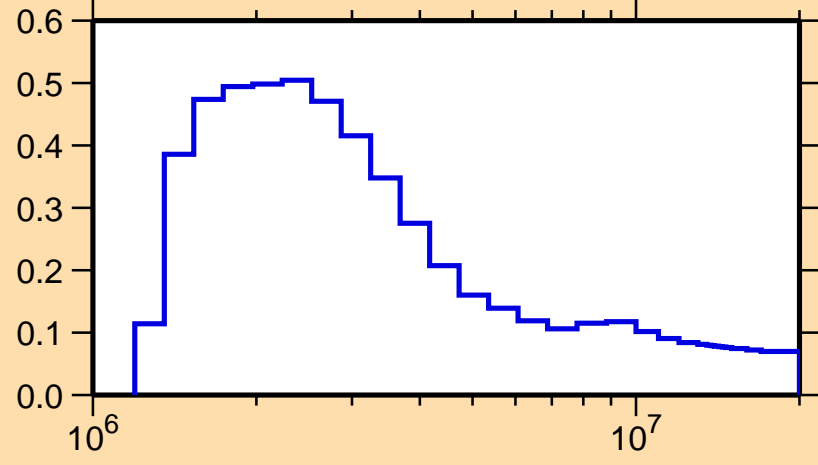
\sigma vs. E for ^{106}\text{Sn}(n,\text{inel.})
