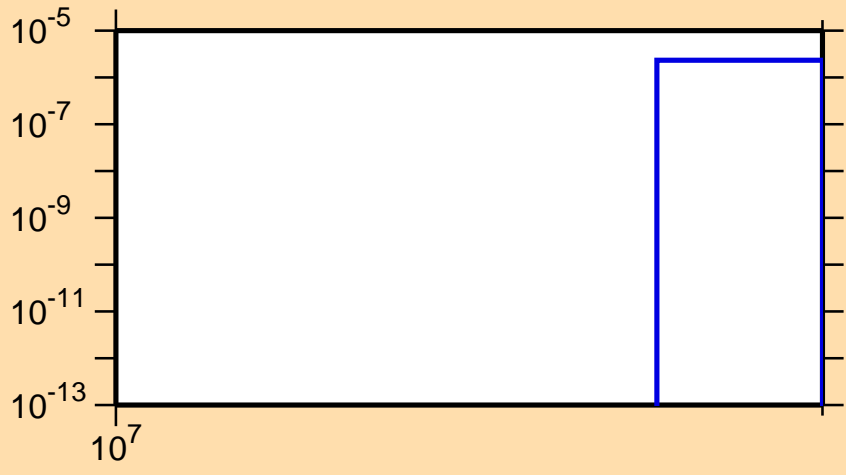
\sigma vs. E for ^{106}\text{Sn}(n,2np)
