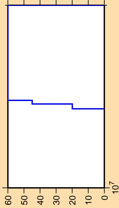
\Delta\sigma/\sigma vs. E for ^{106}\text{Sn} (mt 45)
