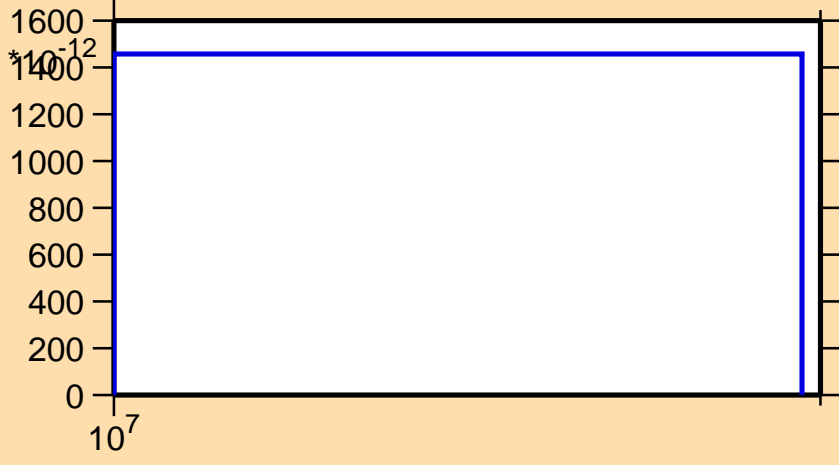
\sigma vs. E for ^{106}\text{Sn}(n,nd)
