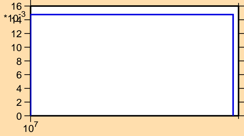
\sigma vs. E for ^{106}\text{Sn}(n,2n)
