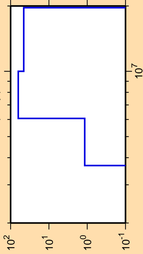
\Delta\sigma/\sigma vs. E for ^{106}\text{Sn}(n,np)
