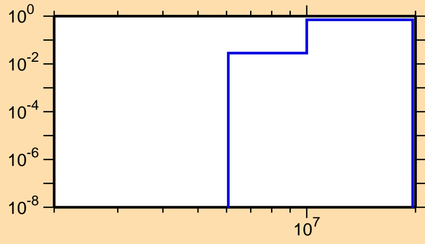
\sigma vs. E for ^{106}\text{Sn}(n,np)
