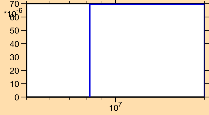
\sigma vs. E for ^{106}\text{Sn}(n,\text{pd})
